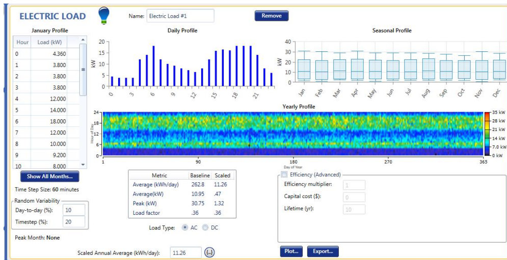
Gambar 7. Beban daya 40 KK
